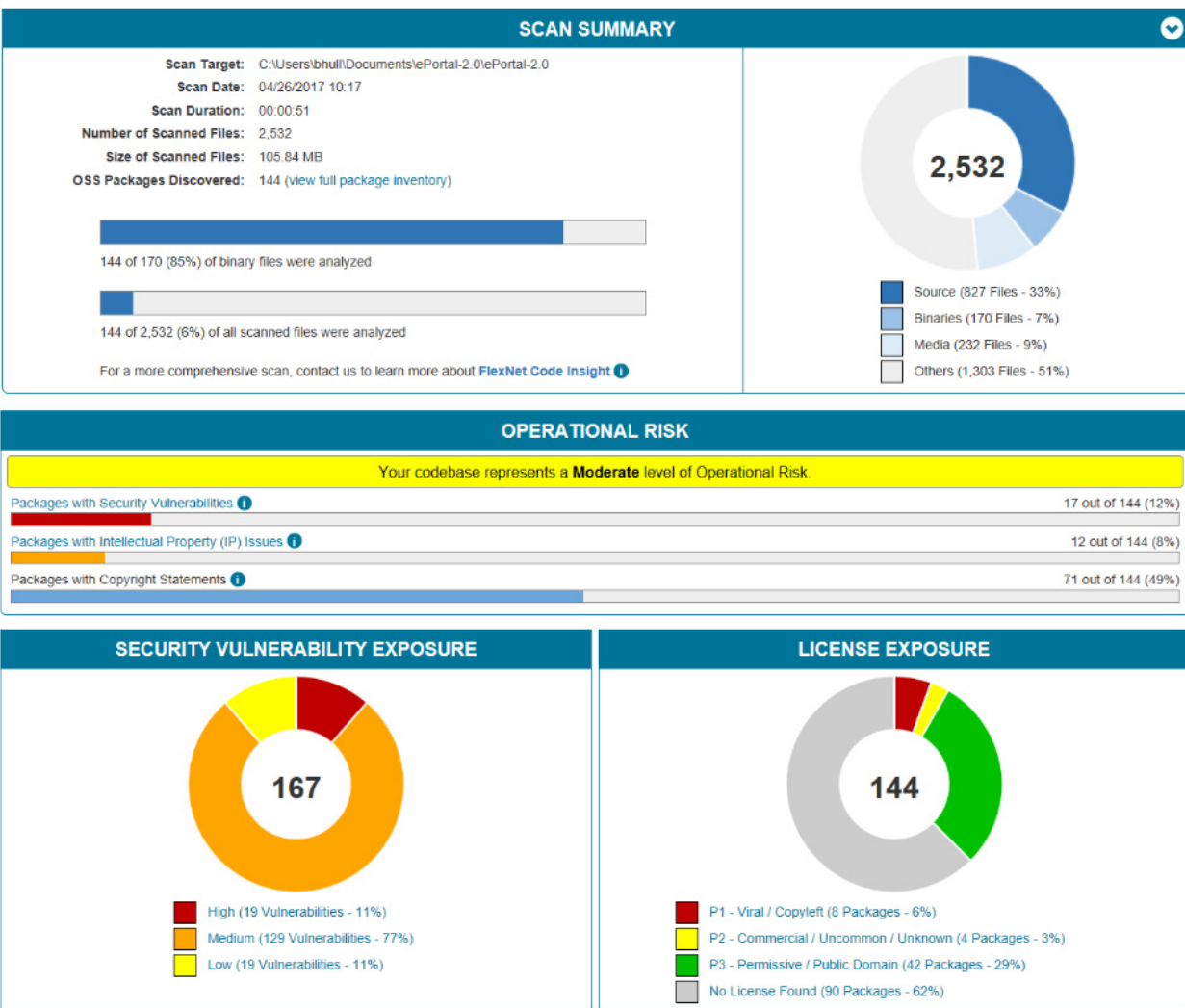
Figure -1: FlexNet Code Aware Initial Summary View
